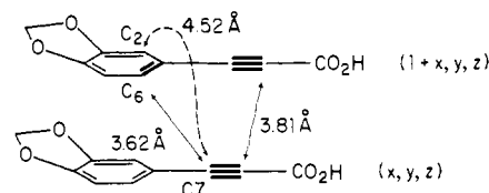
Figure 7. Schematic view of a topochemical Diels–Alder reaction for acid 2a .
